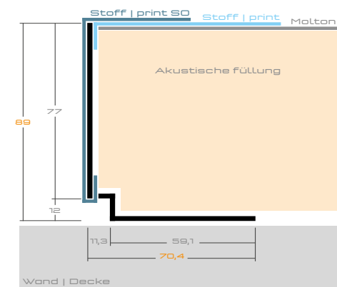
Aluminiumprofil 89 mm
