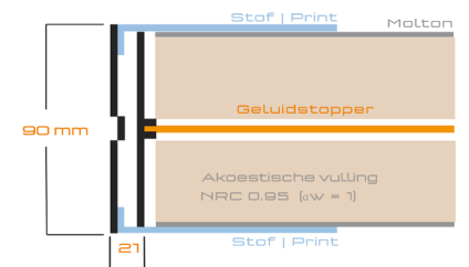
Aluminium profiel 90 mm
